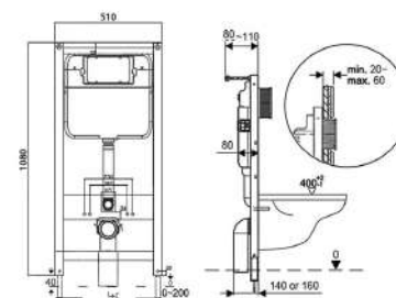
T-8051 Size:1080x510x800mm
