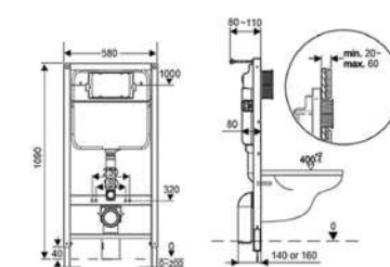
T-8053 Size:1090x580x800mm
